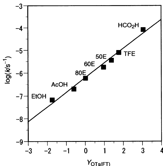
Fig. 1. A plot of \log k against Y_{OTs(FT)} for the solvolysis of 1OTs at 25.0 °C; m = 0.64 ( r = 0.9921 ). For Y_{OTs(FT)} see Ref. 13.
